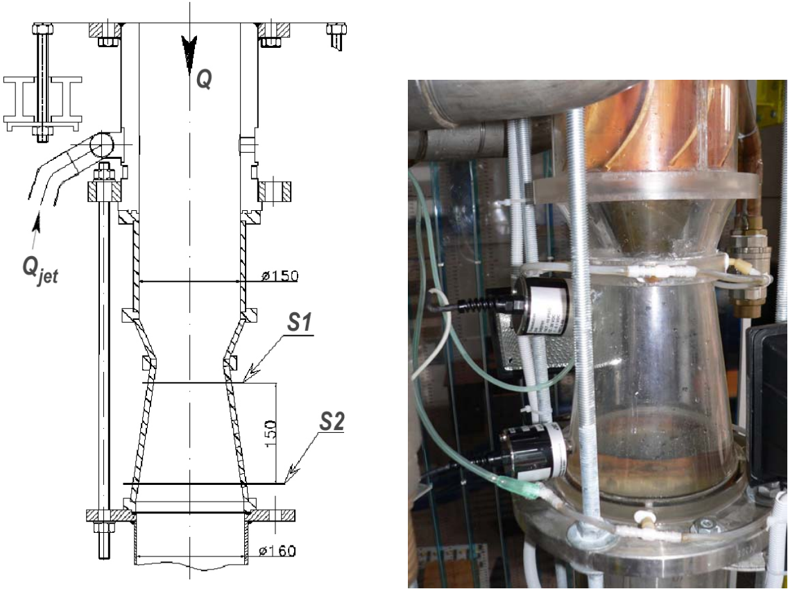
Fig. 5: Pressure transducers mounted on the cone wall
