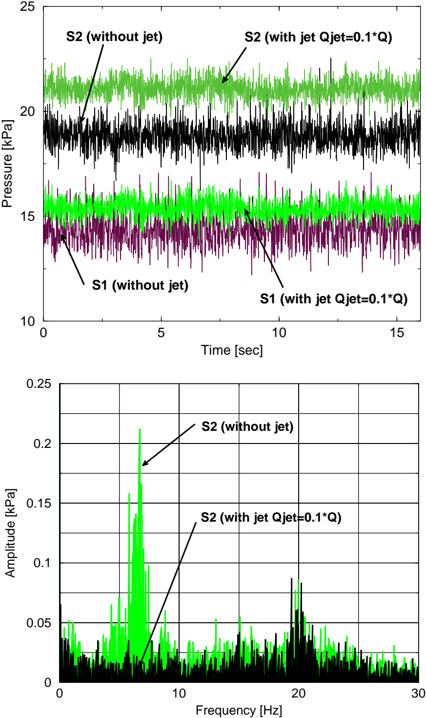
Fig. 6: Unsteady pressure measured on the cone wall in sections S1 and S2 without and with axial jet control (above). Fourier spectrum of the experimental data recorded in section S2 without and with axial jet control (below).
