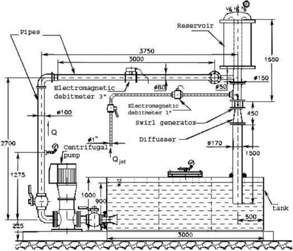
Fig. 1: Closed loop test rig for experimental investigations of swirling flows, at the UPT-NCESCF
