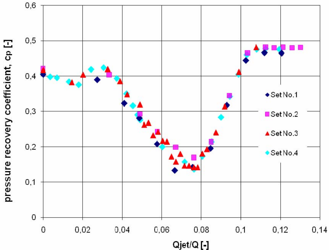
Fig. 7: Pressure recovery coefficient against ratio between axial jet control discharge ( Q_{jet} ) and main flow discharge ( Q ).
