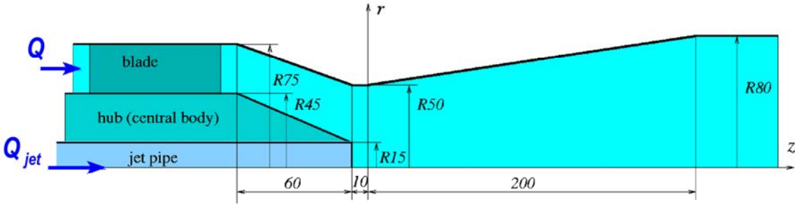
Fig. 3: Meridian cross section of the apparatus for swirling flow generation and analysis in a conical diffuser. Actual dimensions in mm.
