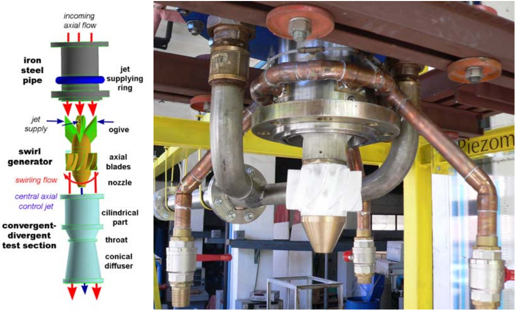
Fig. 2: The swirling flow apparatus designed (left) and installed (right) on the test rig. Axial blades in the upstream annular section provide a controllable swirling flow profile. A tandem of guide vanes and free-wheel runner will be considered in a future
